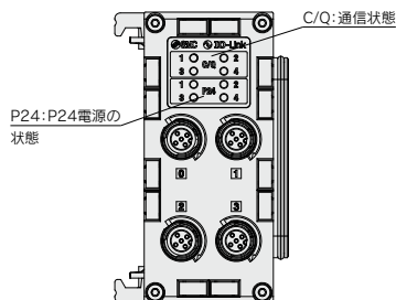
EX600-LBB1
