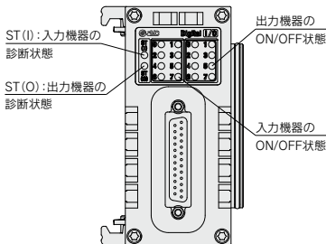
EX600-DM□E
