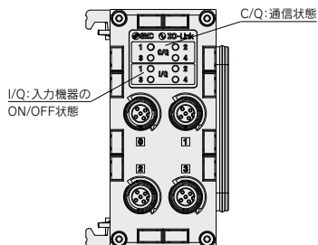
EX600-LAB1
