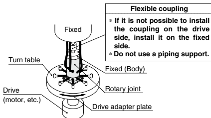
Example of adapter plate drive
