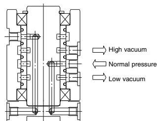
Using normal pressure port
