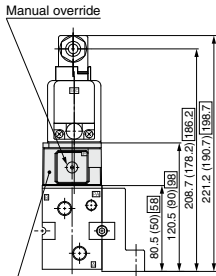
Residual pressure release valve spacer (AZ512-59 A B )
