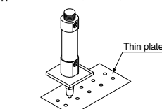
Punching
