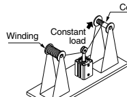
Coil winding
