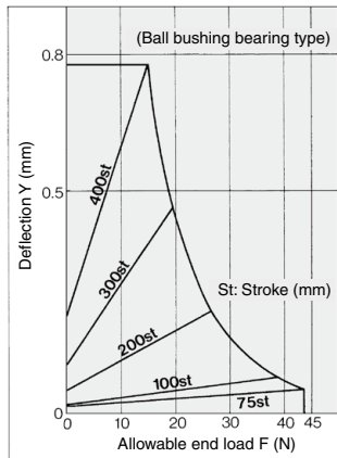
MGCL□20-Stroke-R
