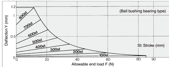
MGCL□40-Stroke-R
