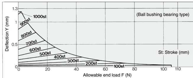
MGCL□50-Stroke-R
