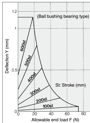
MGCL□32-Stroke-R
