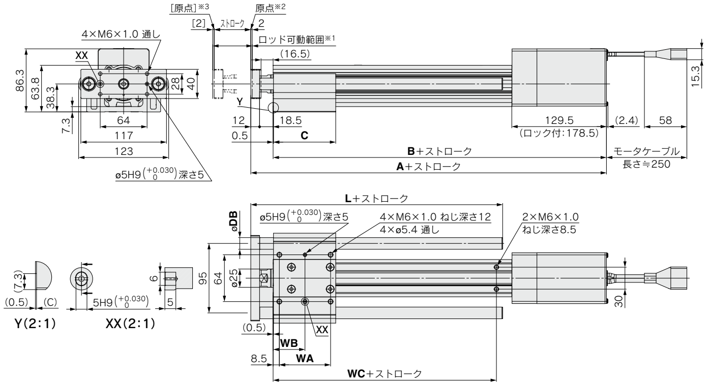
寸法表 LE2YG32D [mm]
