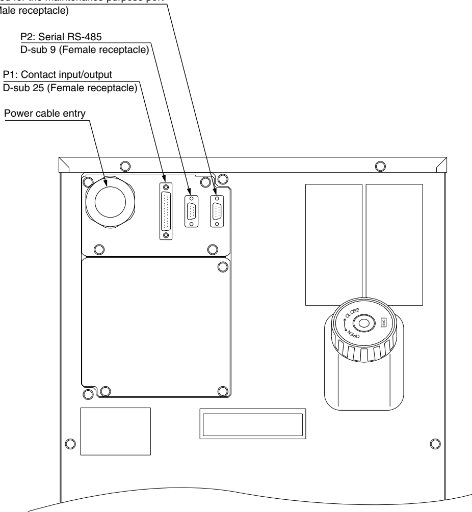
Rear side
