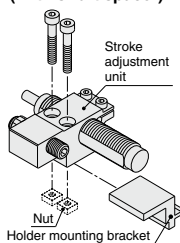
MY2H-A25L2-6-XB20 (With short spacer)
