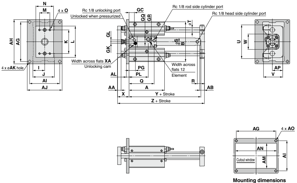
Mounting dimensions
